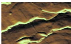
Fig. 2 HAADF-STEM micrograph of the as-bonded Al-Cu wire-bond cross-section
